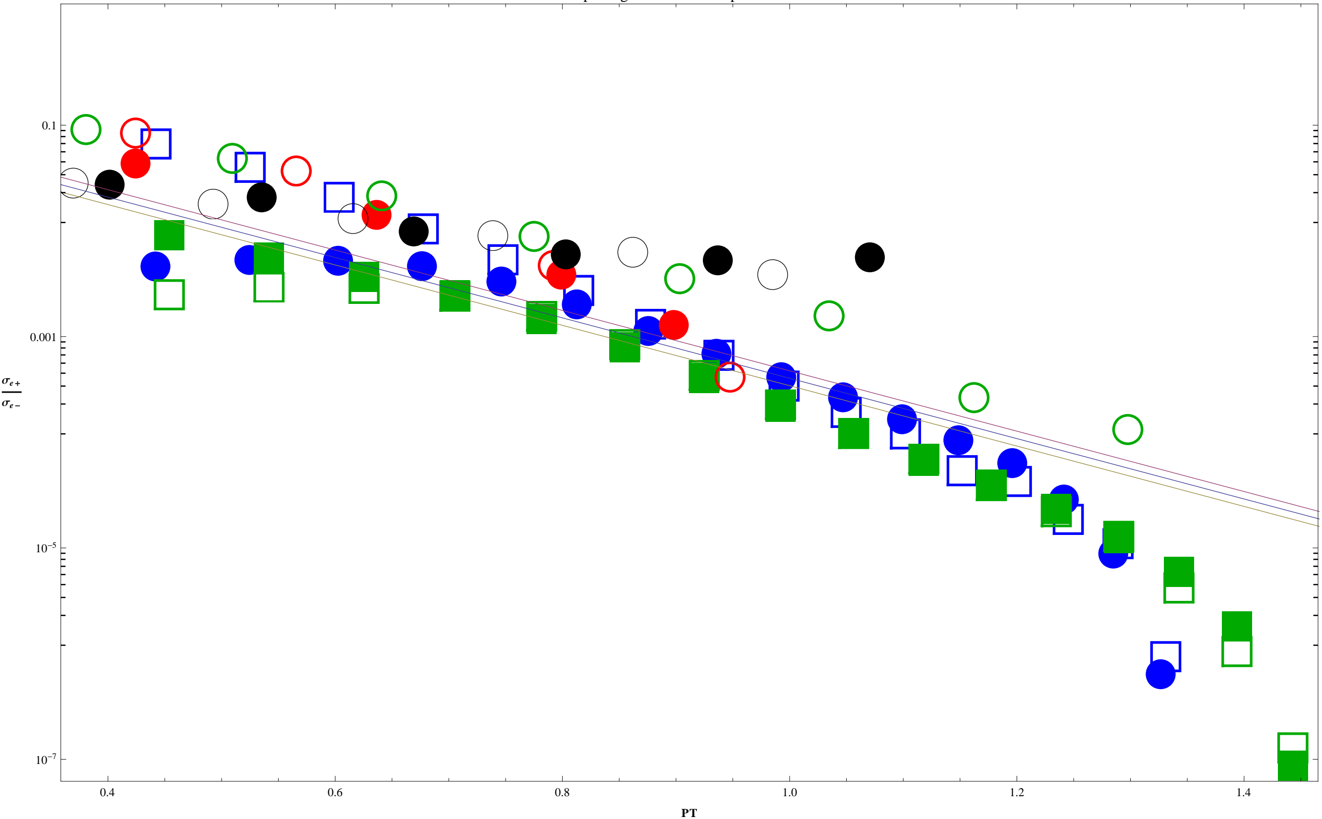
Comparing BETA to Jlab positron data
