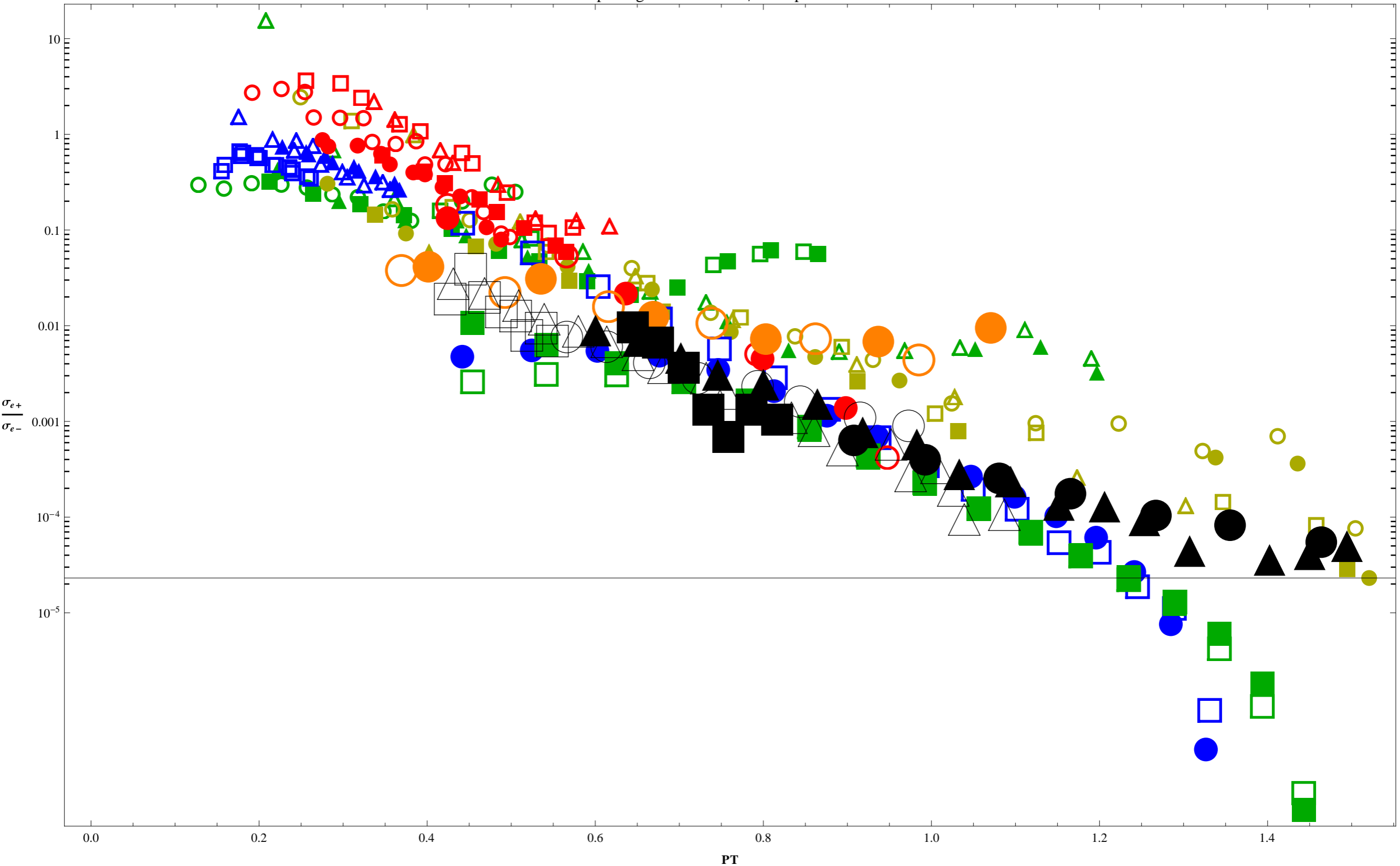
Comparing BETA to Jlab/E143 positron data
