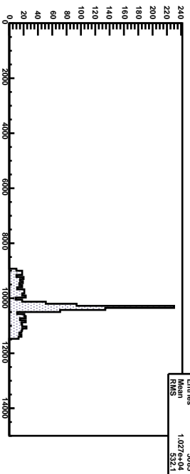
HWCI-07 RAW TDC+
