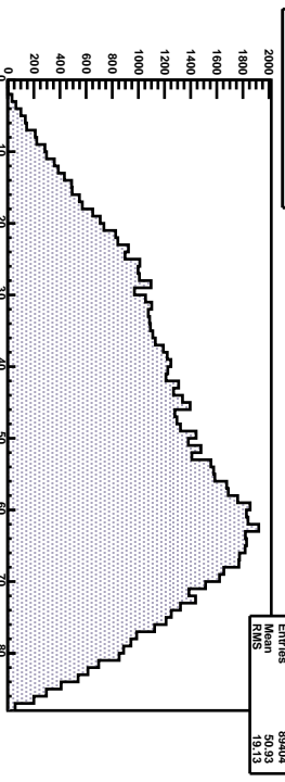
HDCC2v raw hitpat layer-11
