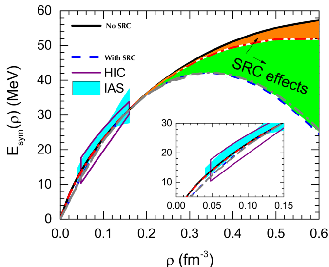
FIG. 5: Density dependence of nuclear symmetry energy E_{sym}(\rho) calculated with and without the SRC high-momentum tail. Constraints on the symmetry energy from analyzing heavy-ion collisions (HICs) and isobaric analog states (IASs) are also shown for comparison. The figure was adapted from [41] and modified by us for clarity.
