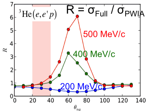
FIG. 13: The calculated {}^3\text{He}(e, e'p) ratio of the cross section which includes rescattering of the struck nucleon (FSI) to the PWIA cross section for p_{\text{miss}} = 0.2 (blue), 0.4 (green), and 0.5 (red) \text{GeV}/c as a function of \theta_{rq} , the angle between the recoil momentum and \vec{q} in the laboratory frame [65].
