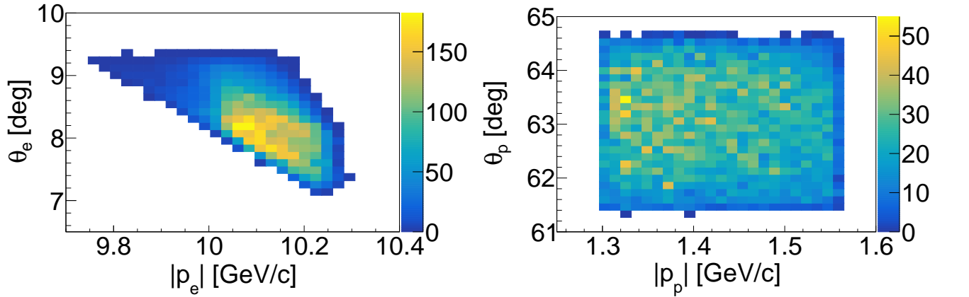
FIG. 16: The angle versus the momentum for the electrons detected in the SHMS (left) and the protons detected in the HMS (right) with cuts as described in Table II for the high- p_{miss} kinematics.
