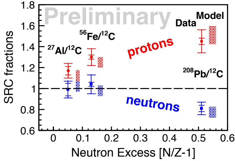
FIG. 3: Red points: The double ratio of the number of (e, e'p) high- p_{miss} (SRC) proton events to low- p_{miss} (mean field) proton events for nucleus A relative to Carbon plotted versus the neutron excess of nucleus A . Red boxes: the prediction of the phenomenological np -dominance model. Blue points and boxes: the same for neutrons.
