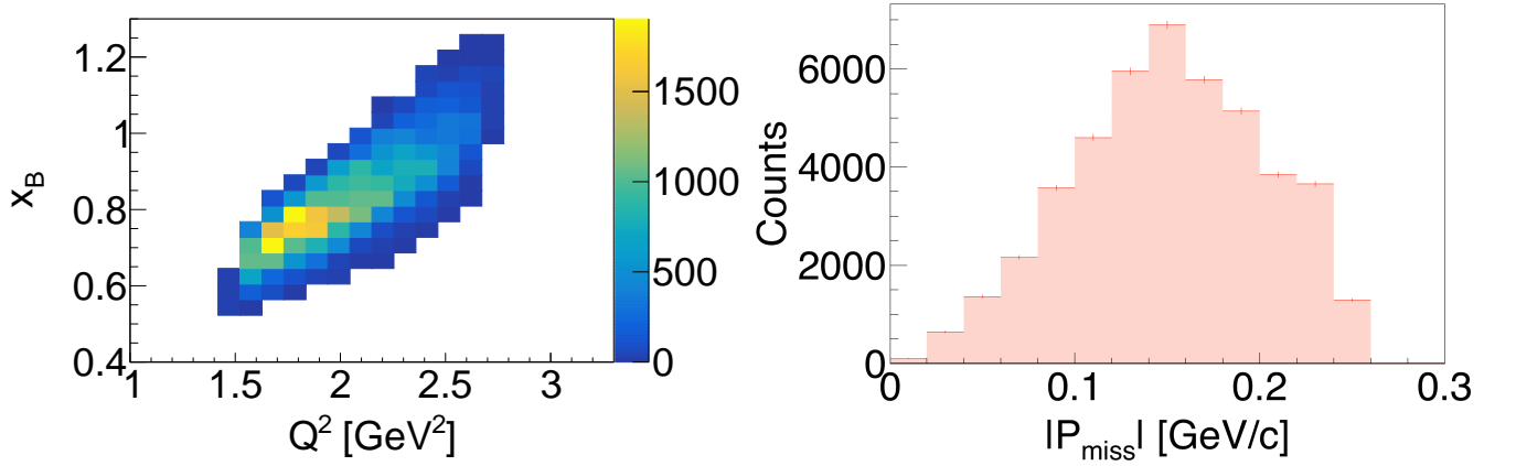
FIG. 15: On the left the x_B scaling variable versus the momentum transfer, Q^2 is shown. On the right, the expected missing momentum distribution is shown for the low- p_{miss} kinematics.
