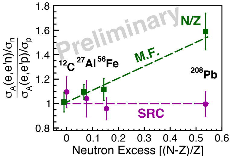
FIG. 2: The A(e, e'p)/A(e, e'n) reduced cross-section ratio for low- p_{miss} (mean-field) [green squares] and high- p_{miss} [SRC] (purple circles) events plotted versus neutron excess. The dashed lines are simple model predictions for the N/Z neutron excess-dependence of the Mean-Field nucleons and the independence of neutron excess of the SRC nucleons.
