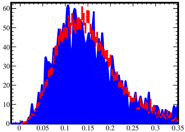
Missing Momentum (GeV/c)
