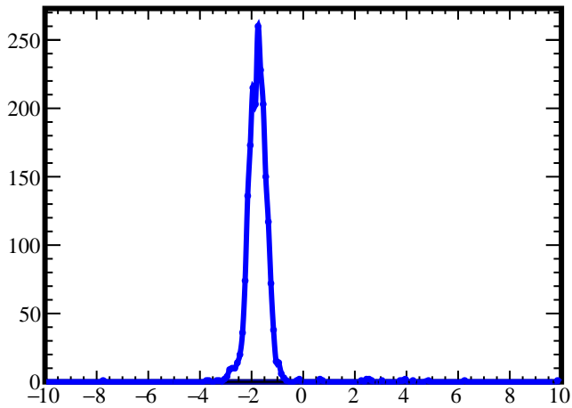
Corrected Cointime (ns)
