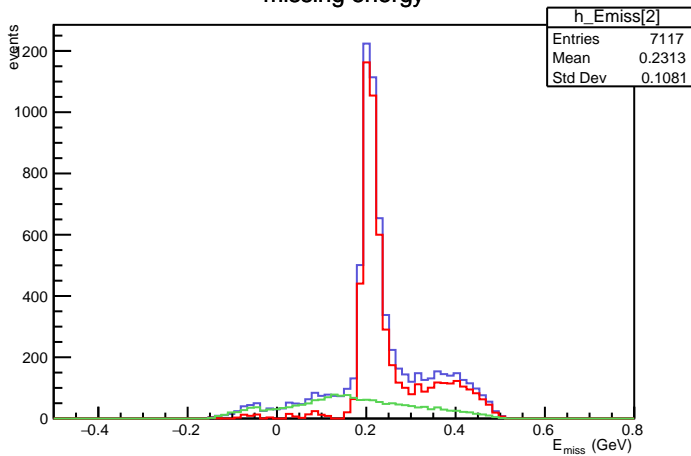
missing energy
