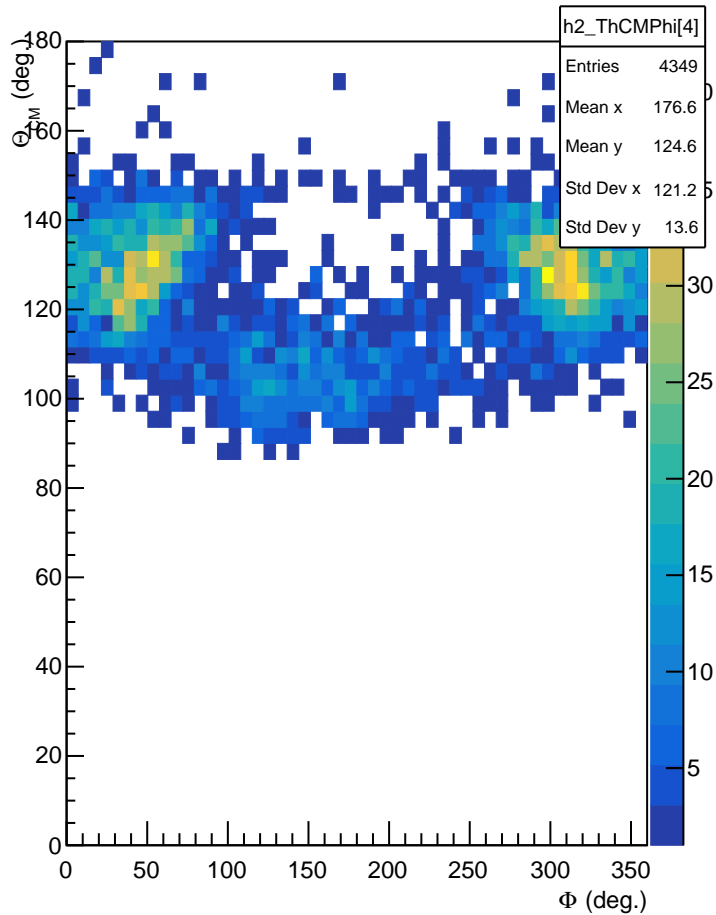
\Theta_{\text{CM}} vs \Phi
