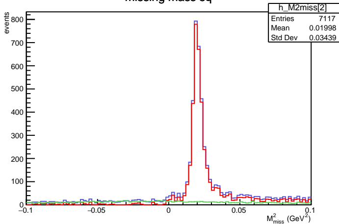
missing mass sq
