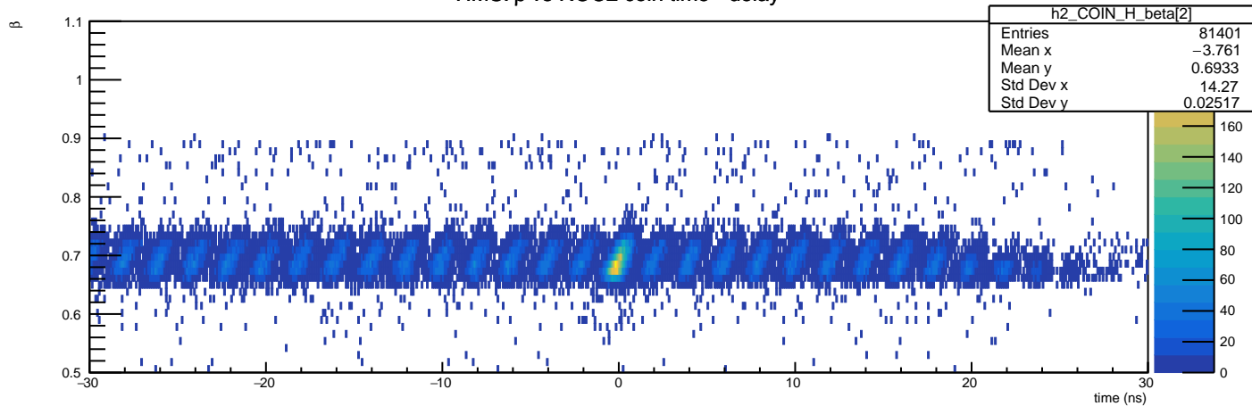
HMS: \beta vs ROC2 coin time - delay
