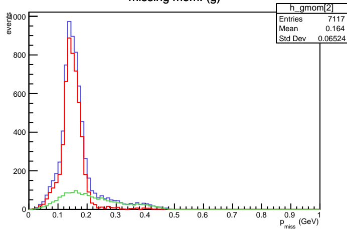
missing mom. (g)
