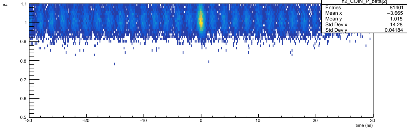
SHMS: \beta vs ROC2 coin time - delay
