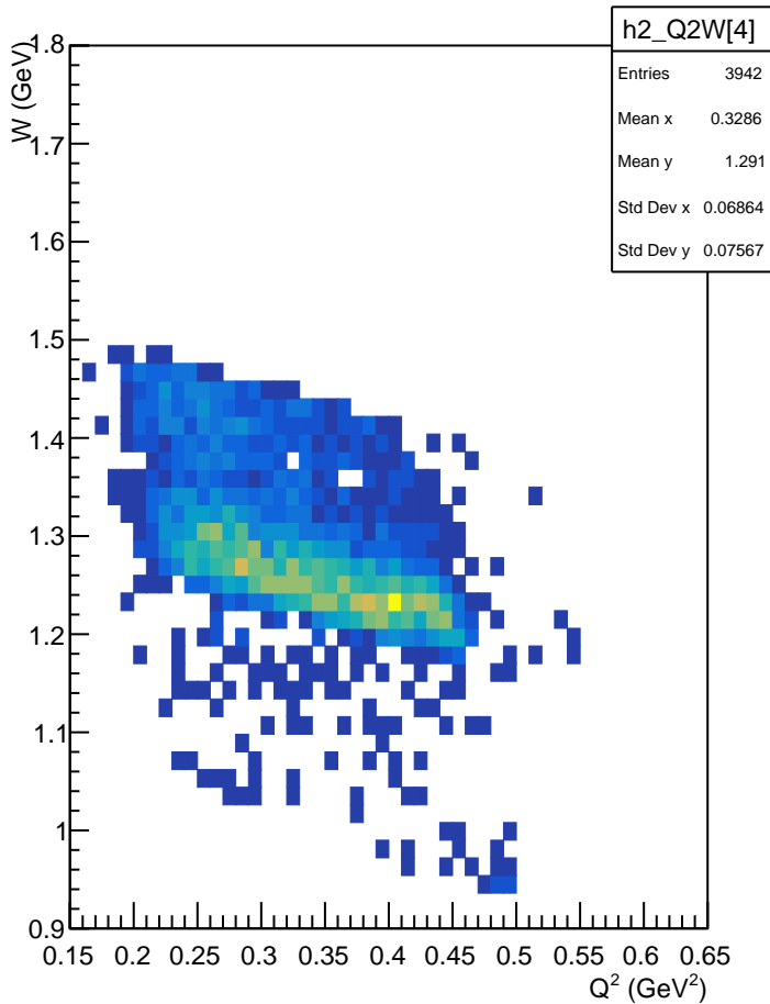
W vs Q 2
