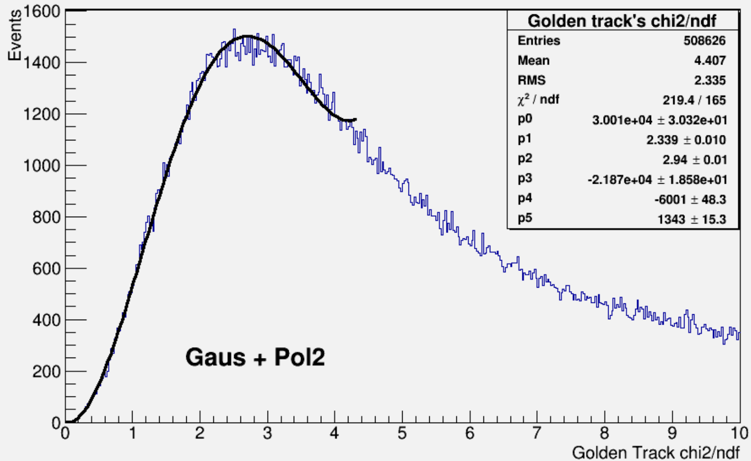
Golden track's chi2/NDF. Run 52949
